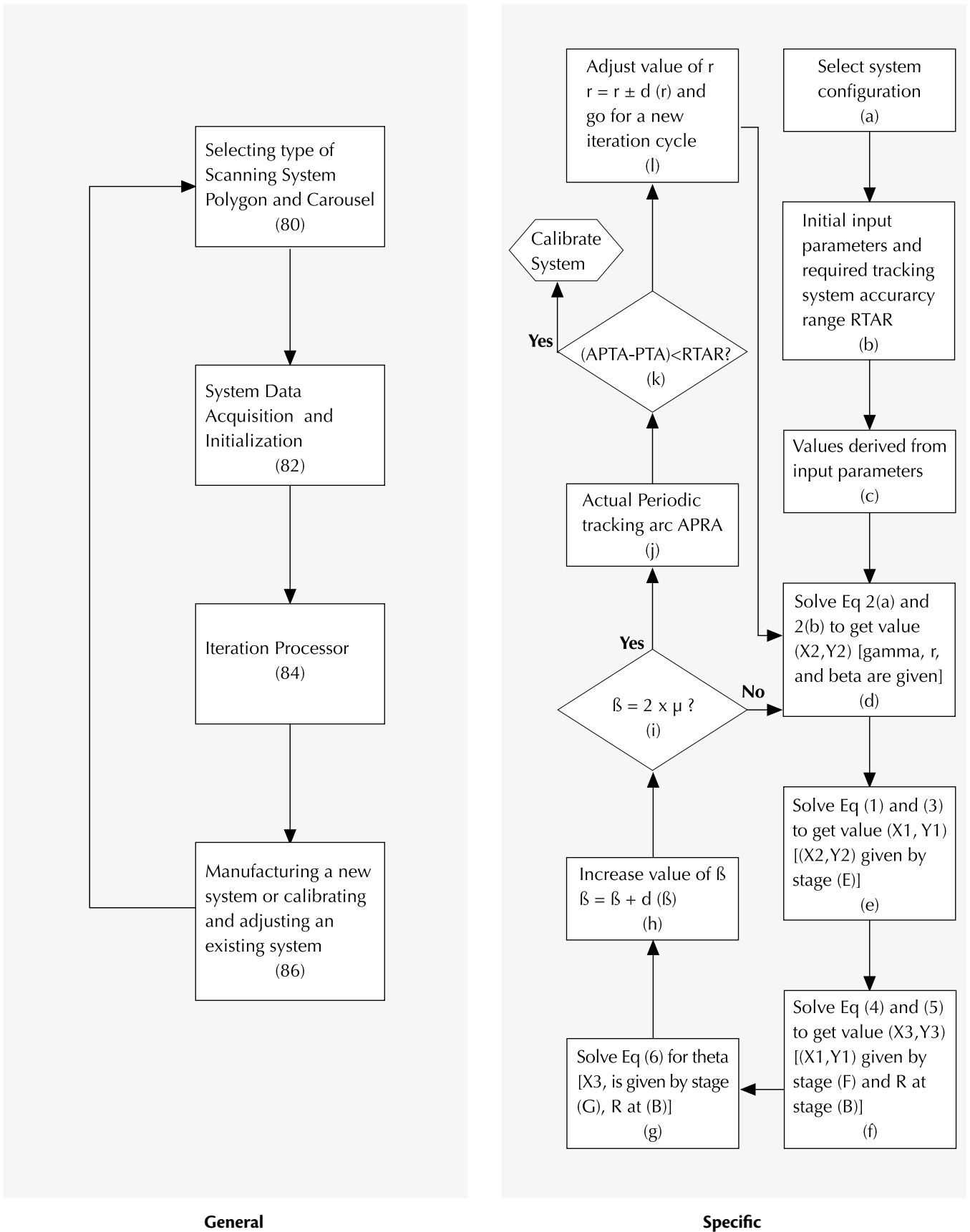
Fig. 8B—Software Flowcharts
